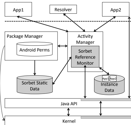
Fig. 3. SORBET architecture: SORBET’s additions to Android are shaded; arrows indicate interactions between components; and dashed arrows are present in Android but unneeded in SORBET.
