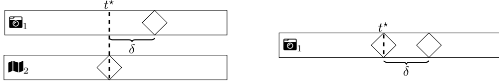
(a) Reference-point-based temporal misalignment. The reference point t^* is the ideal sampling time for both sensors. Sensor S_1 samples at time t^* + \delta , while sensor S_2 samples at the reference point t^* . The temporal misalignment of sensor S_1 is \delta , while the temporal misalignment of sensor S_2 is 0.
