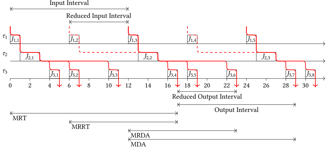
Fig. 7: Updated End-to-End latency definitions without imbalance in the input and output intervals. Again, arrows indicate data flow, and dashed lines indicate that data is overwritten before being read by the subsequent task.
