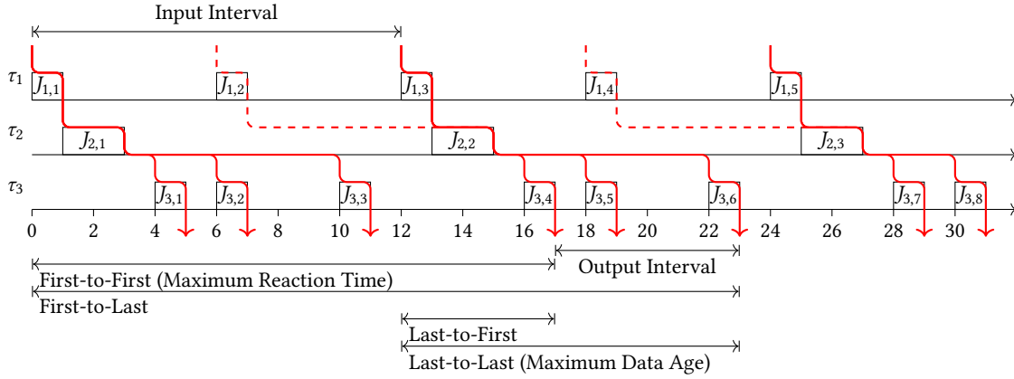
Fig. 6: End-to-end latency semantics formulated in [14]. Arrows indicate data flow. Dashed lines indicate that data is overwritten before being read by the subsequent task.
