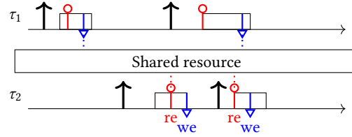
Fig. 4: Communication between tasks.
