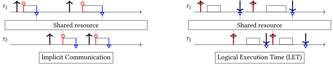
Fig. 5: Implicit communication (left) and LET communication (right).
