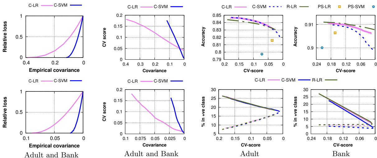
(a) Loss vs. Cov. (b) Cov. vs. CV score (c) Single binary sensitive attribute
