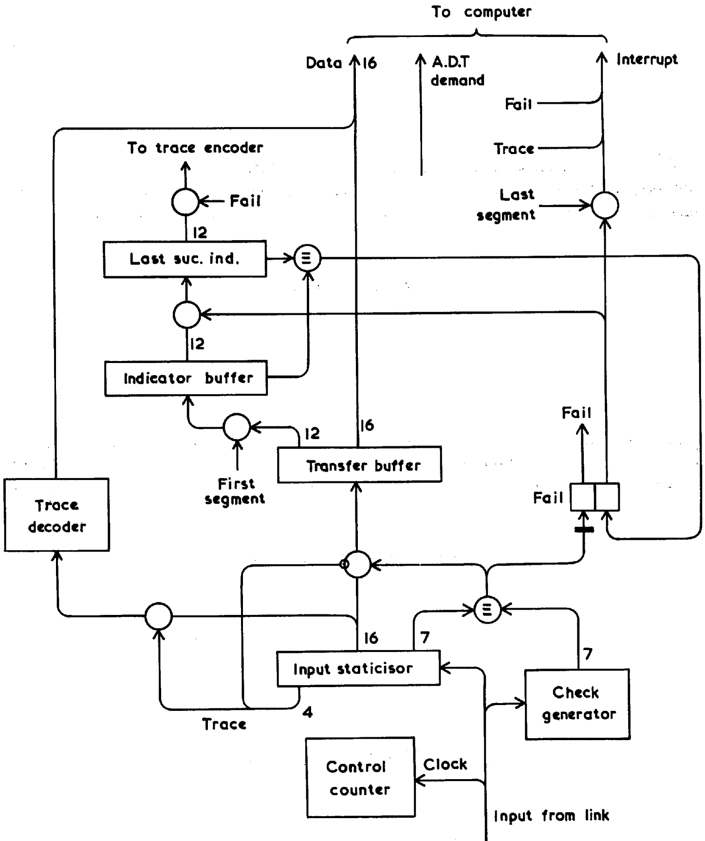
FIG. 4 SCHEMATIC DIAGRAM OF LINK HARDWARE (INPUT)
