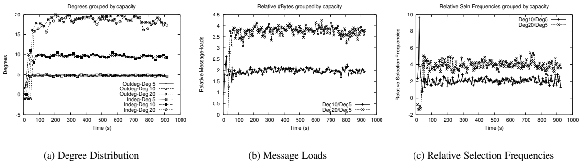
Figure 8: PlanetLab 250 nodes with high churn and moderate capacity distribution
