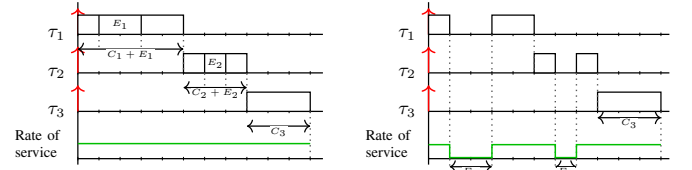
Fig. 5: Schedule with overruns and schedule with blackout. Red arrows represent task arrivals.
