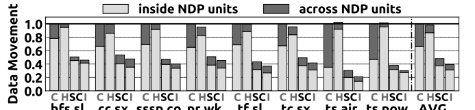
Figure 15: Data movement in real applications for C: Central , H: Hier , SC: SynCron and I: Ideal .
