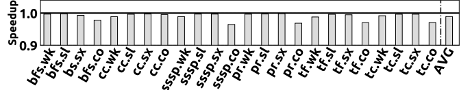
Figure 20: Speedup of SynCron normalized to flat with 40 ns link latency between NDP units, under a low-contention and synchronization non-intensive scenario.
