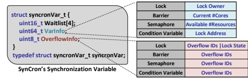
Figure 9: Synchronization variable of SynCron ( synchronVar ).
