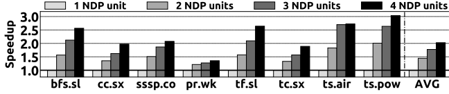
Figure 13: Scalability of real applications using SynCron .
