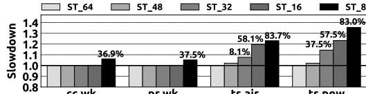
Figure 22: Slowdown with varying ST size (normalized to 64-entry ST). Numbers on top of bars show the percentage of overflowed requests.
