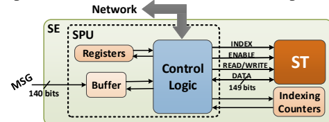
Figure 6: The Synchronization Engine (SE).
