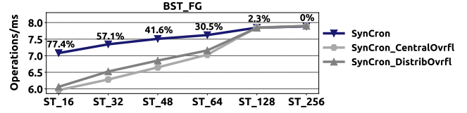
Figure 23: Throughput achieved by BST_FG using different overflow schemes and varying the ST size. The reported numbers show to the percentage of overflowed requests.
