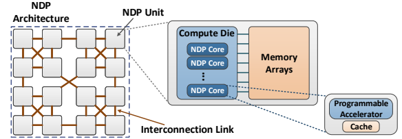
Figure 1: High-level organization of an NDP architecture.
