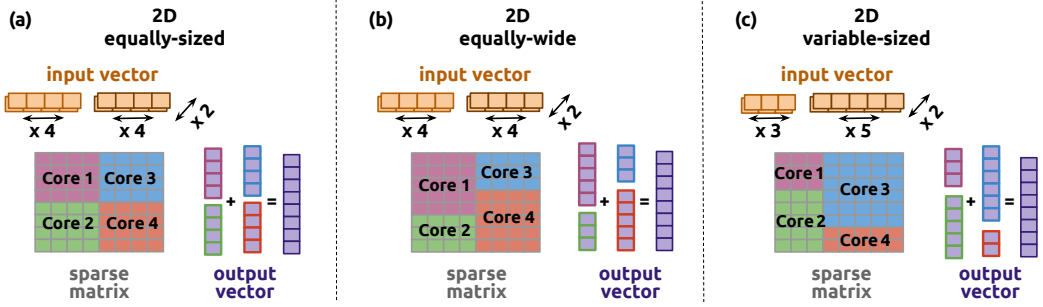
Fig. 8. The 2D partitioning techniques of SparseP package assuming 4 PIM cores and 2 vertical partitions.
