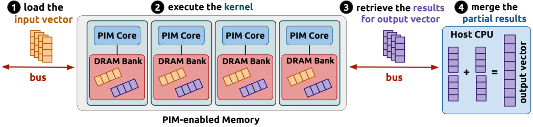
Fig. 4. Execution of the SpMV kernel on a real PIM system.
