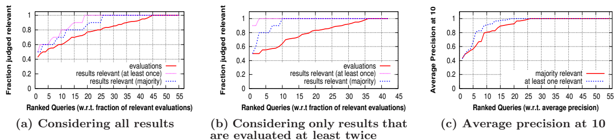
Figure 1: Fraction of evaluations / individual Cognos results that were judged relevant (queries ranked w.r.t. fraction of relevant judgments) (a) considering all results, and (b) considering only those results for a query, which were evaluated at least twice; (c) Average precision for the top 10 results returned by Cognos
