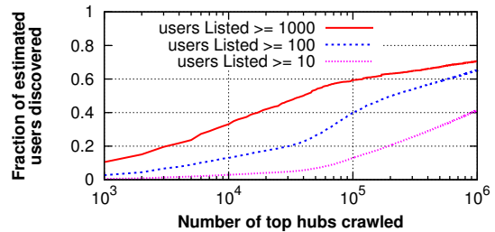
Figure 2: Fraction of estimated number of experts who are included in at least K Lists, that is discovered in the hub-based crawl, for K = 10, 100, 1000 .
