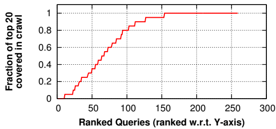
Figure 3: Distribution of the fraction of Twitter WTF top 20 results that is covered in our hub-based crawl (for the queries discussed in Section 5.3.3)
